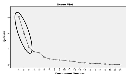
Gambar 2: Scree Plot Daya Saing
