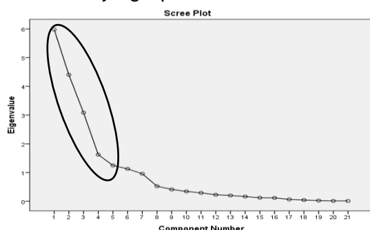
Gambar 1: Scree Plot Modal Insan
