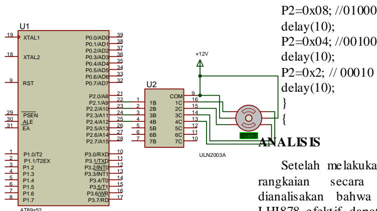
Gambar 5. Driver Motor Stepper
